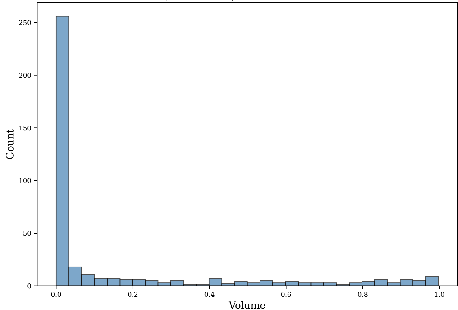
Volume Distribution of Downsampled Sequences (Filtered >20 seqs per motif) sigma: (1, 1) | volume: (0.1, 0.5)
